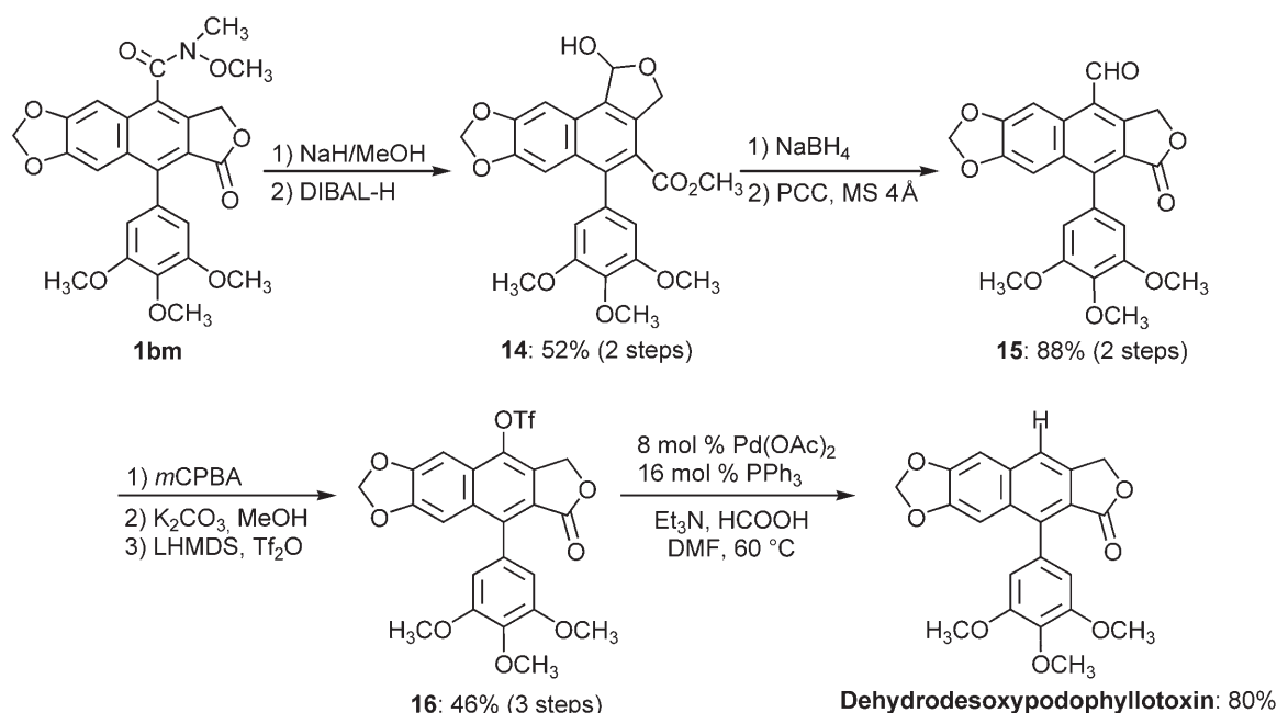
Scheme 9. Total synthesis of dehydrodesoxypodophyllotoxin.
