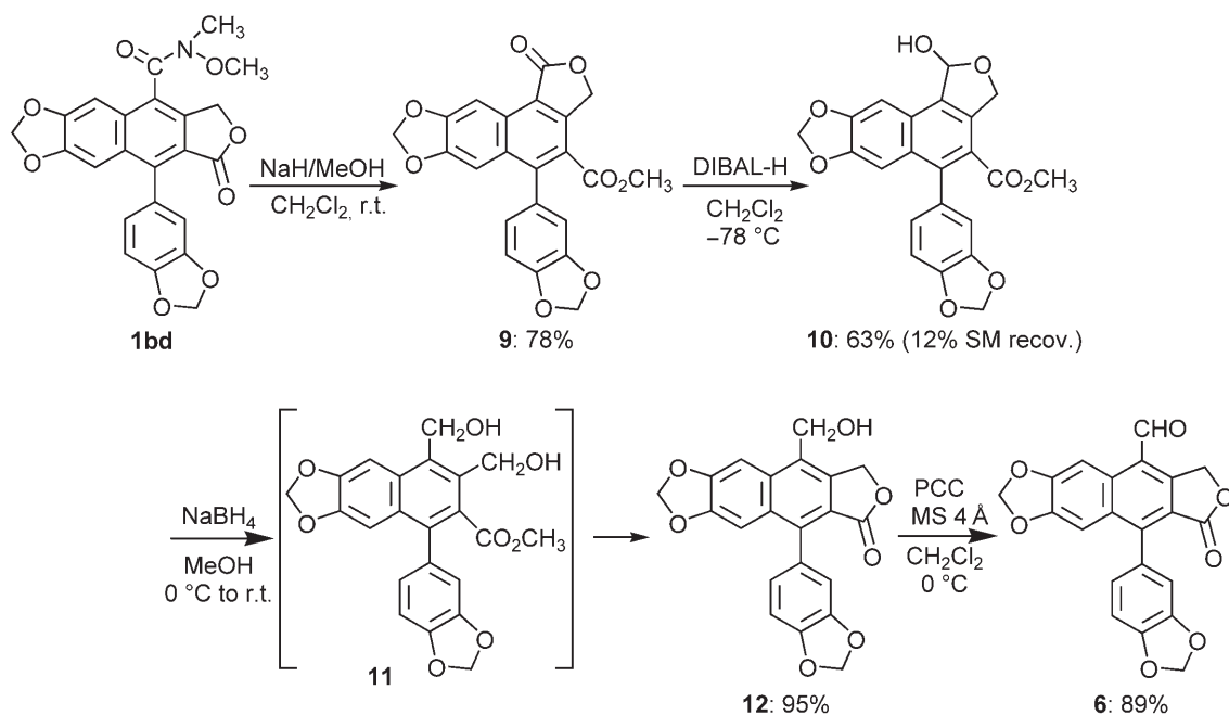
Scheme 6. Conversion of 1bd into aldehyde 6 .
