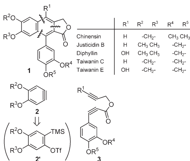
Figure 1. Plan for syntheses of aryl-naphthalene lignans.
