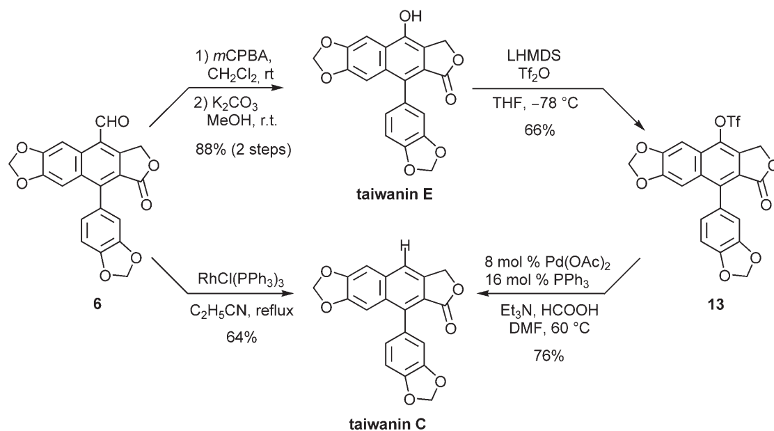
Scheme 7. Total syntheses of taiwanins C and E.
