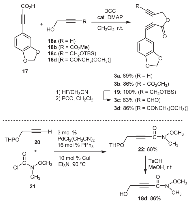
Scheme 10. Synthesis of substrates 3a–d.
