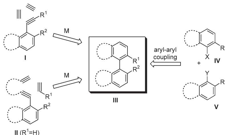
Scheme 1. Synthesis of biaryls via [2 + 2 + 2] cocyclization.
