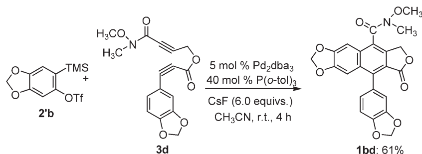
Scheme 4. [2+2+2] Cocyclization of diyne 3d and aryne precursor 2'b .
