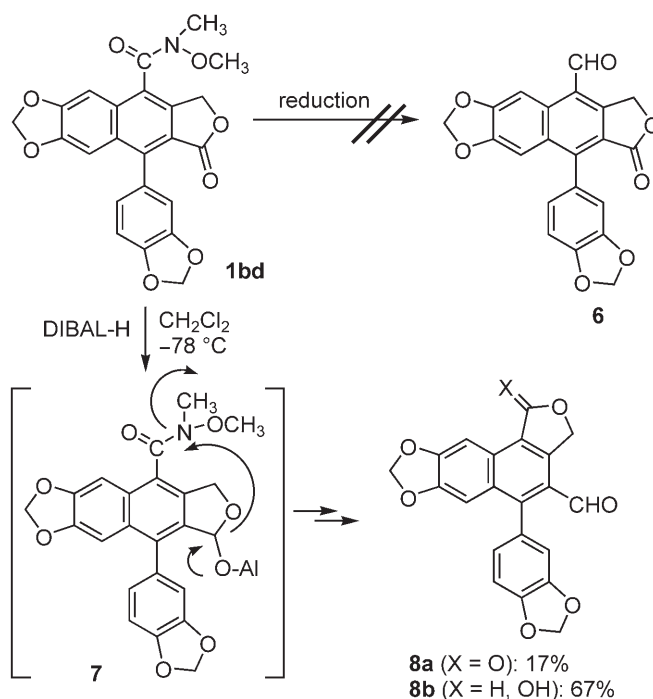
Scheme 5. Attempts at conversion of 1bd into aldehyde 6 .
