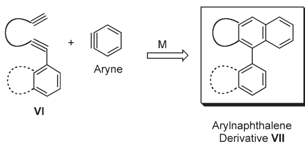
Scheme 2. Plan for [2+2+2] cocyclization of diynes and arynes.
