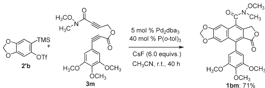
Scheme 8. [2+2+2] Cocyclization of diyne 3m and aryne precursor 2'b .
