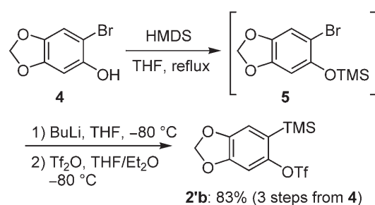
Scheme 3. Synthesis of aryne precursor 2'b .
